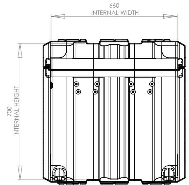
SECTION Z-Z SCALE 1 : 12
