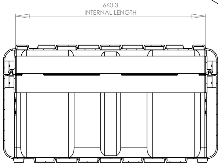
SECTION Y-Y
