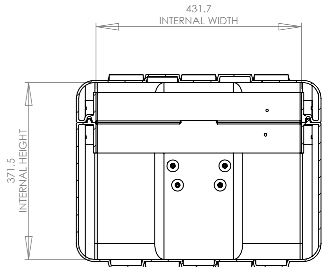
SECTION Z-Z
