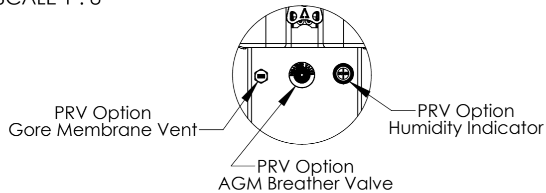
SECTION Y-Y SCALE 1 : 8
